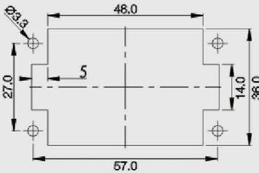
面板安装开孔图 Panel cut out
