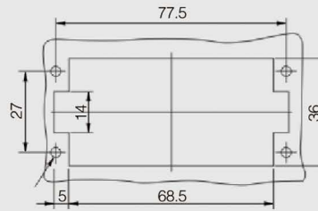
面板安装开孔图 Panel cut out
