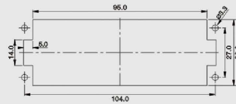
面板安装开孔图 Panel cut out
